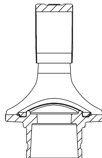
SECTION Q-Q
