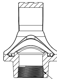
SECTION K-K 1.5" FNPT
