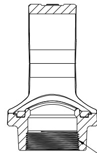
SECTION P-P 2' FNPT
