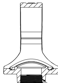
SECTION R-R 2" FNPT
