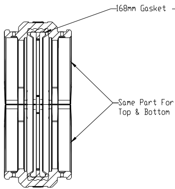
SECTION E-E
