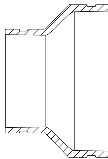
SECTION E-E
